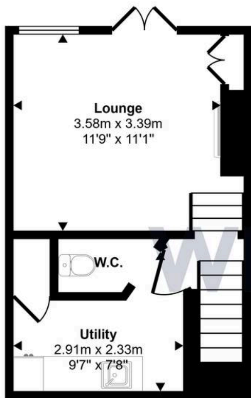
Lower Ground Floor Approx 24 sq m / 262 sq ft
