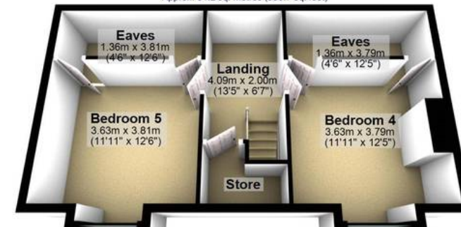
Second Floor Approx. 51.2 sq. metres (550.7 sq. feet)
