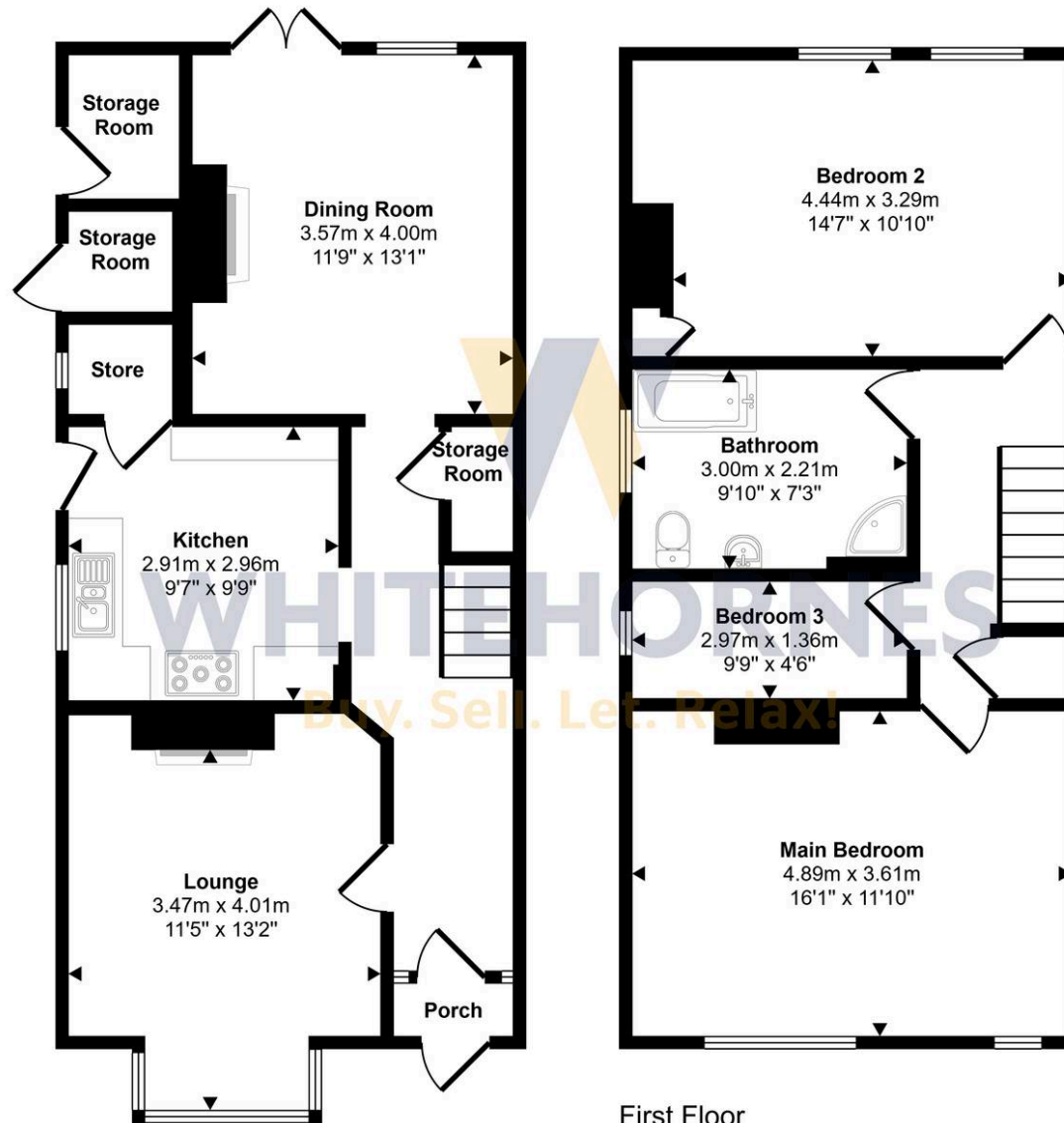
First Floor Approx 53 sq m / 574 sq ft
